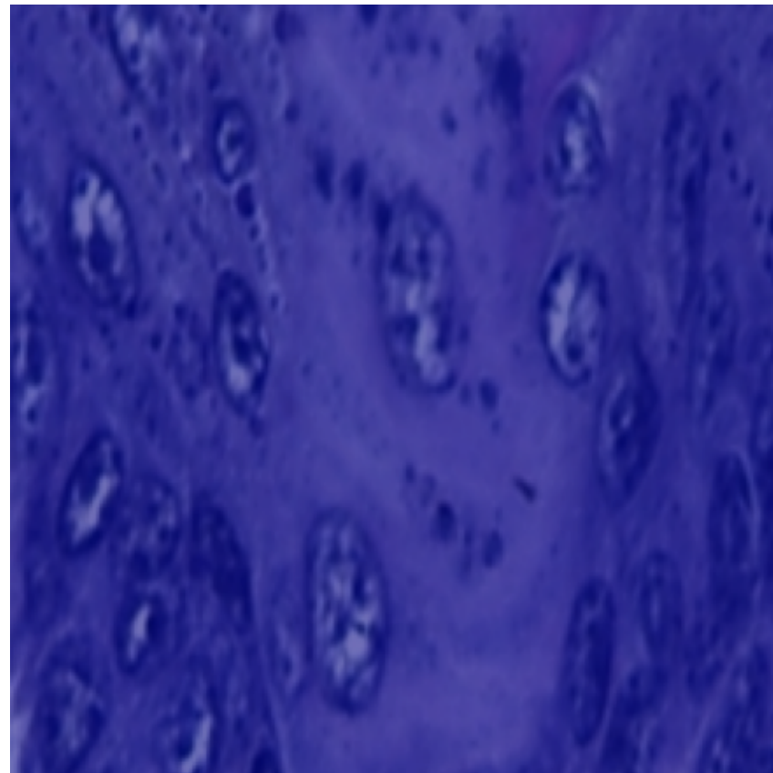
Grad-CAM: Healthy 99.51%
