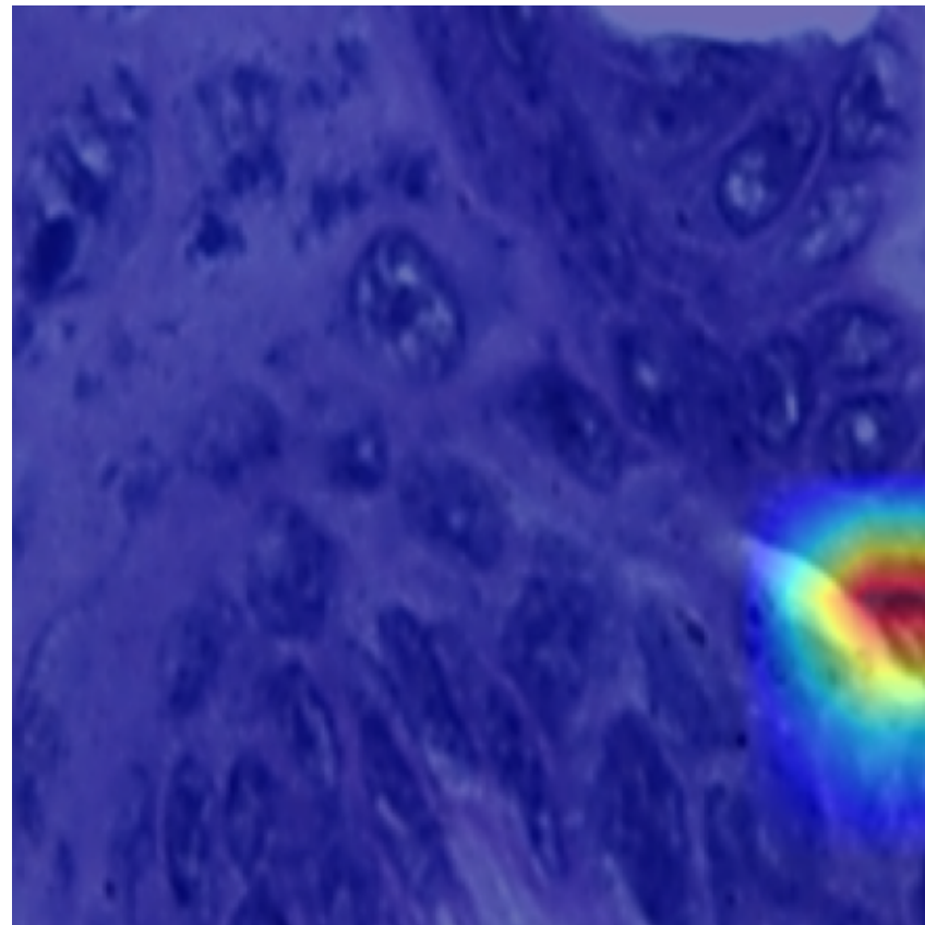
Grad-CAM: Healthy 98.26%
